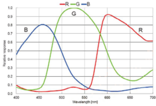
Quantum Efficiency Curve for Mono and Color
