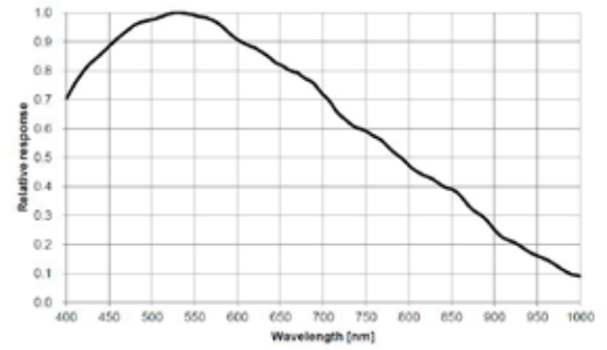
Quantum Efficiency Curve for Mono Sensor
