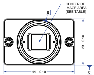
CS MOUNT
