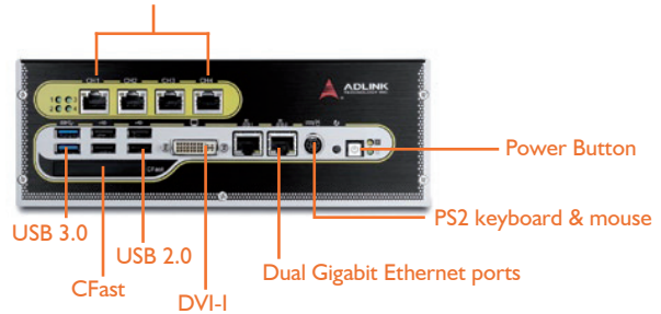
EOS-I200 Front View
