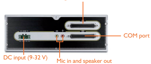
EOS-I200 Back View
