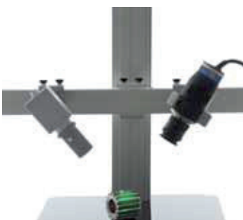
90° configuration with zero distortion macro lenses.
