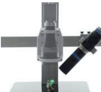
Bi-telecentric lenses used for both projection and vision.
